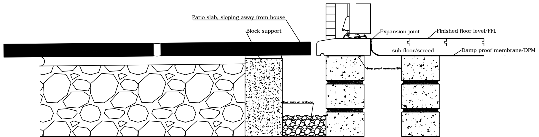
Valdi Ltd - Front Door and French Doors - Standard Timber Drip Sill - Inward Opening Raised level entry suggested construction detail.
