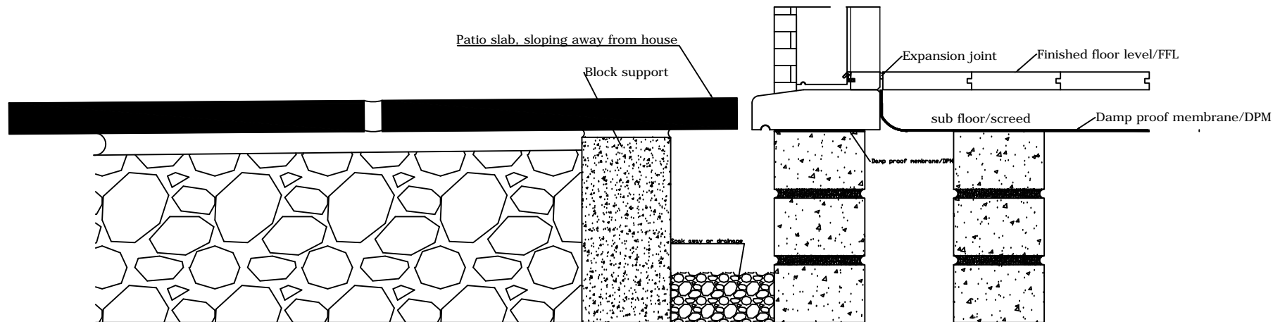
Valdi Ltd - Front Door and French Doors - Standard Timber Drip Sill - Outward Opening Raised level entry suggested construction detail.
